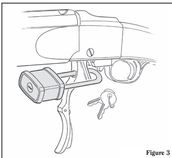
Correct Installation of Lock For Ruger® No. 1® Rifles Only
